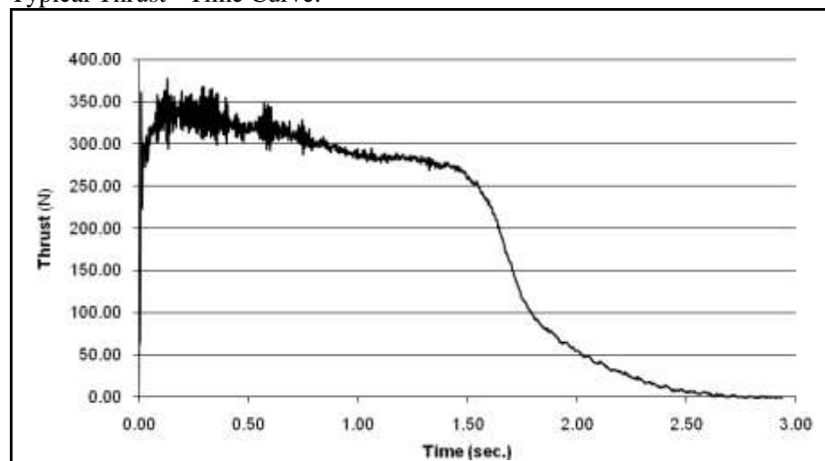
Typical Thrust - Time Curve:
